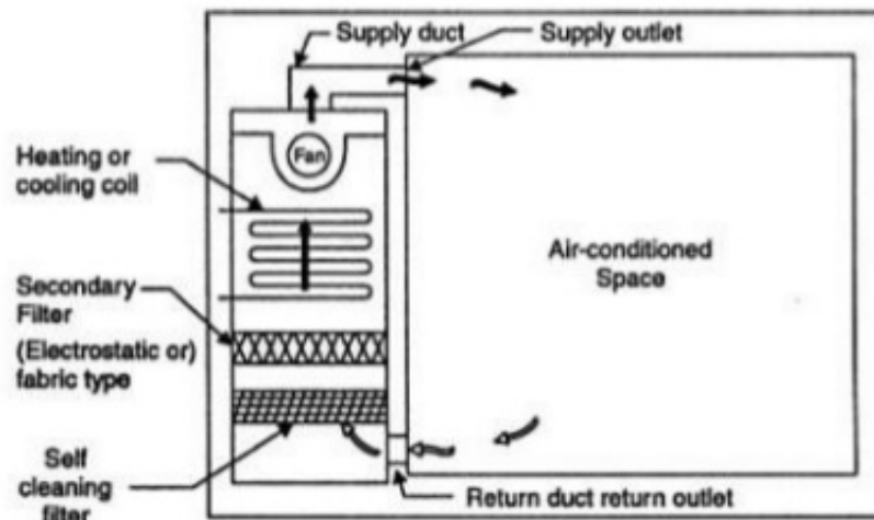
Fig. 27.1. Air-conditioning cycle.
