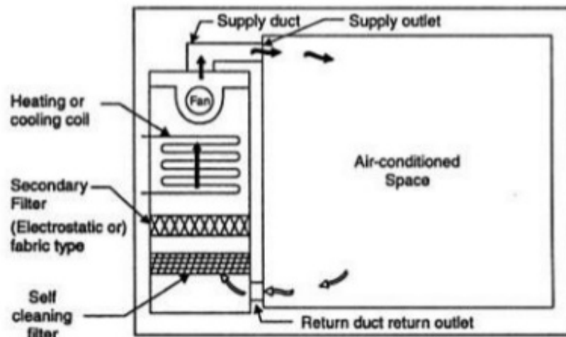
Fig. 27.1. Air-conditioning cycle.
